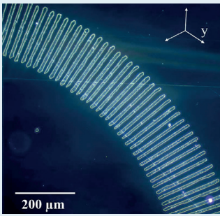
LiNbO 3 wafer structured by maskless poling
